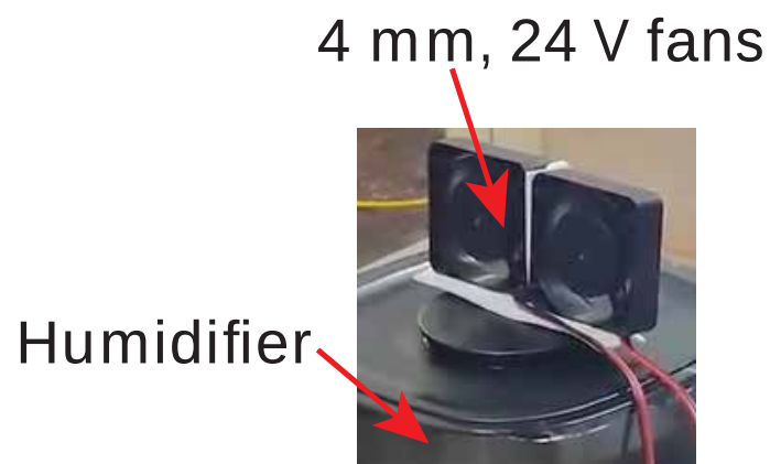
Figure 12. The humidifier with the fans near the vents
